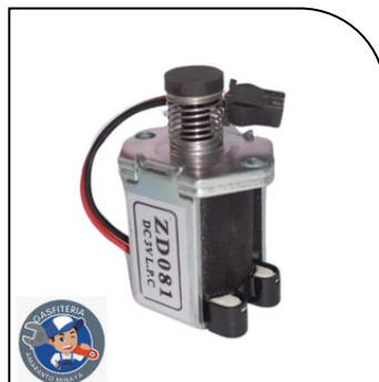
VALVULA SELENOIDE VITALITY STANDAR
