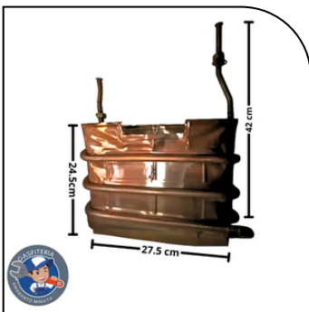
SERPENTIN SPLENDID MASTER 13 L
